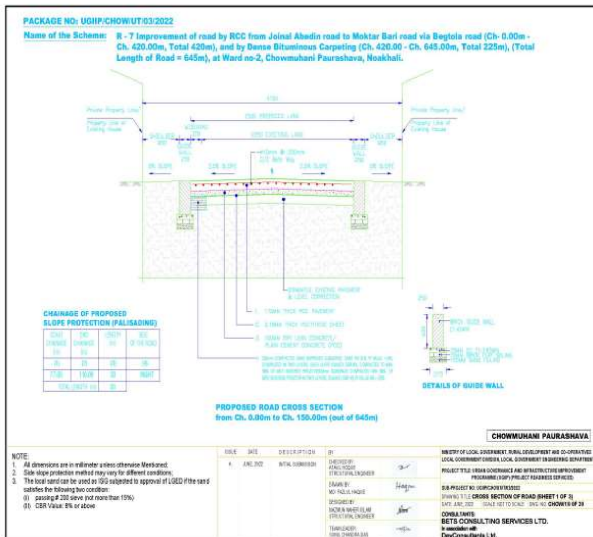
Figure 3: Cross-Section of Road
